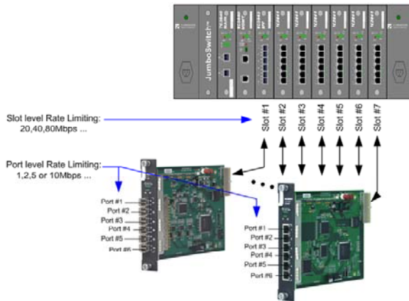
Fig. 4 JumboSwitch on Rate Control
