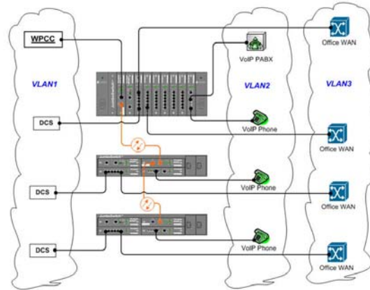
Fig. 3 VLAN Concept
