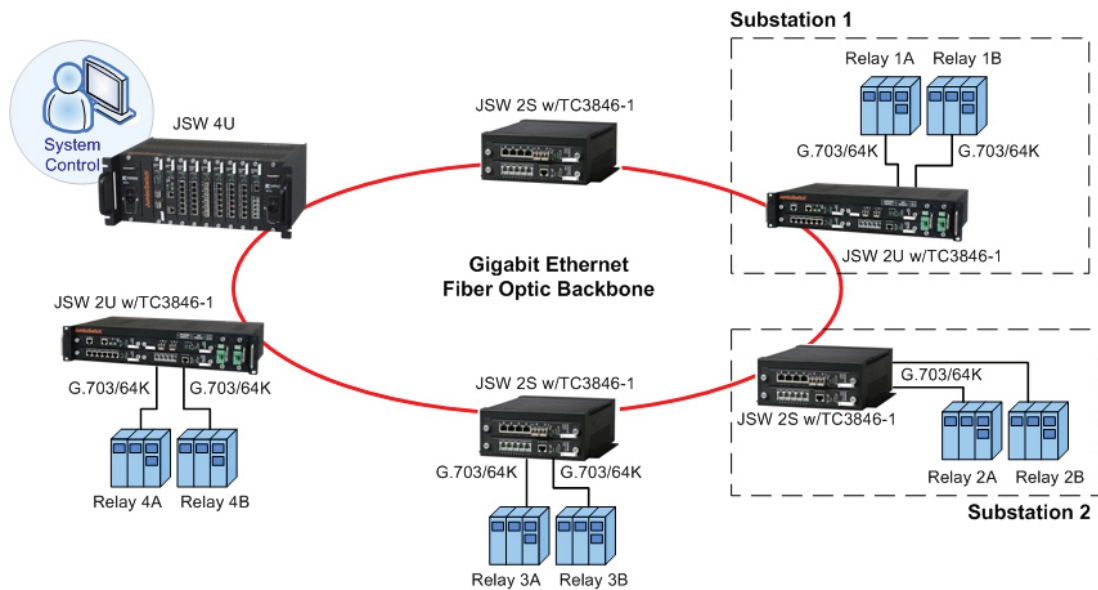
Typical Teleprotection Application Using TC3846-1 to Extend G.703/64K (Co-Directional) over Ethernet Network
